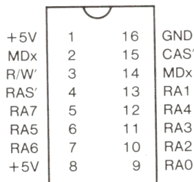
Figure 7-8 The 64K RAM Pinouts
